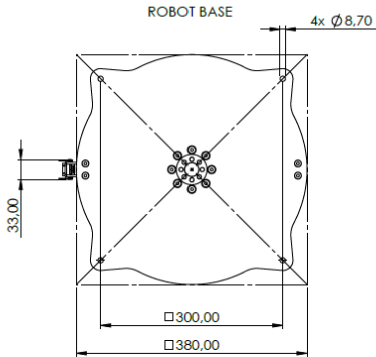
Base drilling pattern of HORST1000
